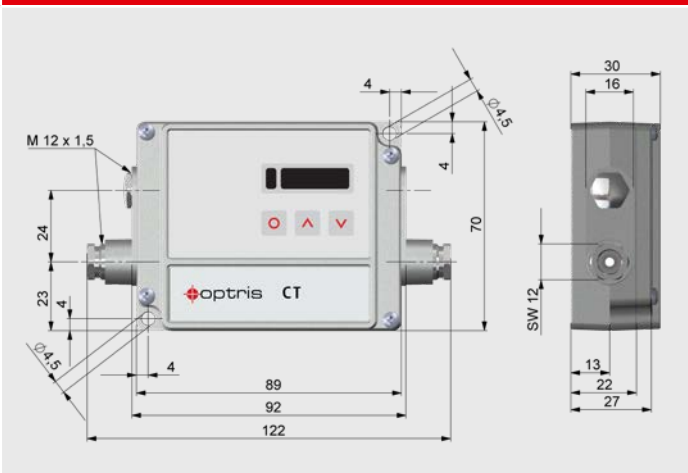
Dimensions electronics
