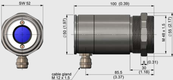
Sensing head
