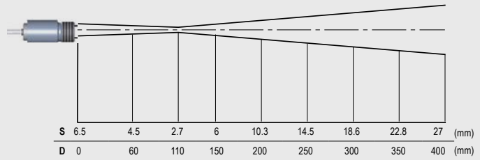
CTi 2ML CF, D:S = 40:1 (Fernfeld = 12:1)
