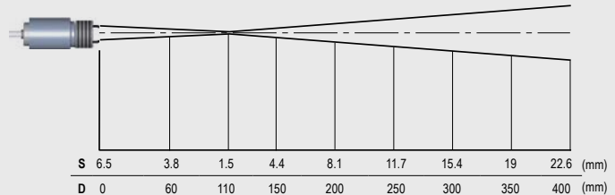
CTi 2MH/2MH1 CF, D:S = 75:1 (far field = 14:1)
