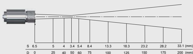
CF optics D:S = 15:1 (far field = 5:1)
